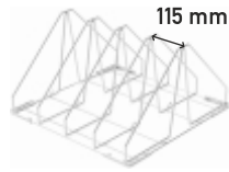
8080-0023 STAINLESS STEEL RACK FOR 4 GN 500x500x170 mm
