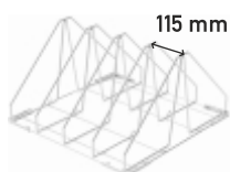
8080-0023 BASE FOR 4 GN STAINLESS STEEL 500x500x170 mm
